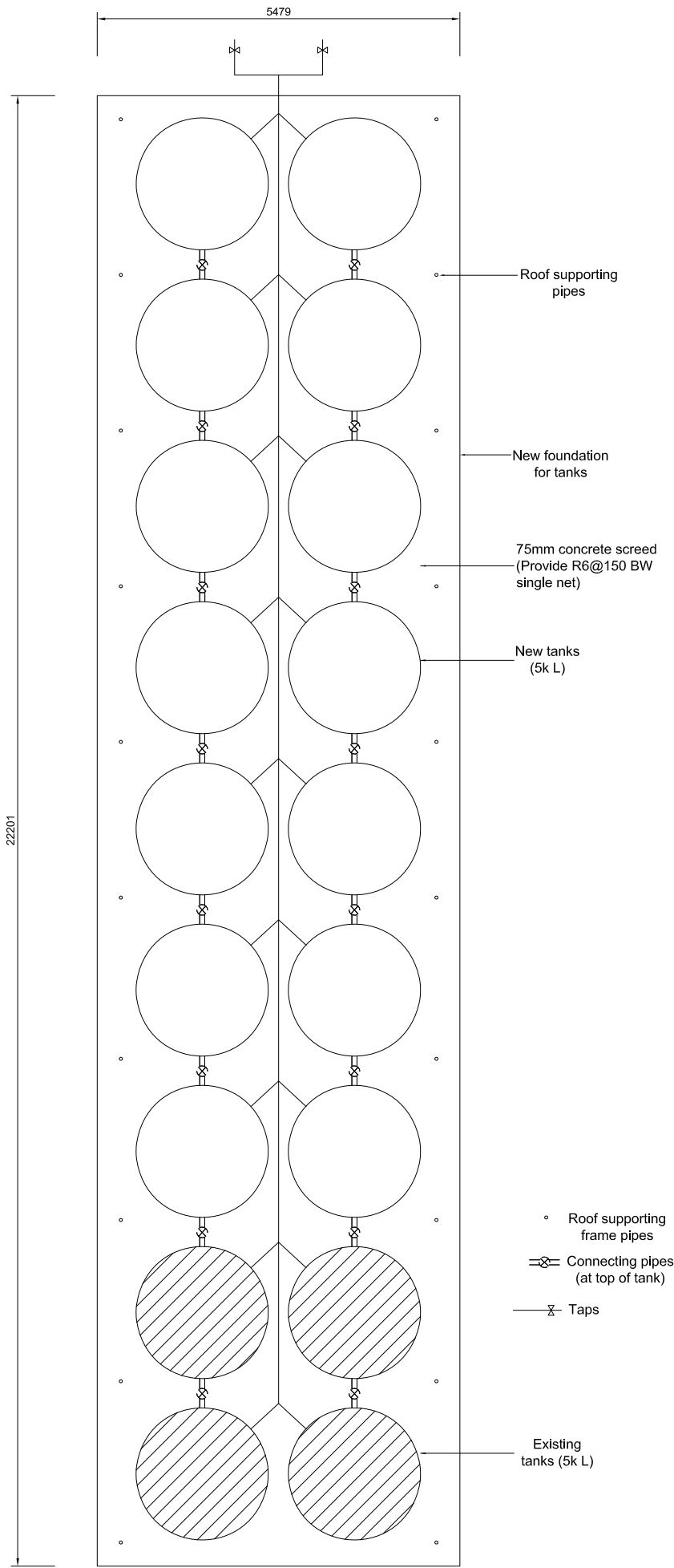
WATER TANK ARRANGEMENT - PLAN OFFICE SITE
