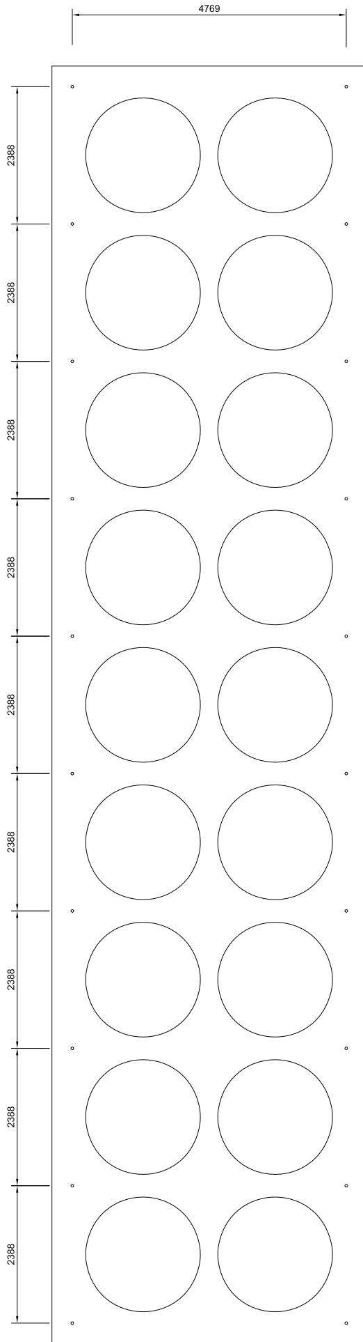
ROOF SUPPORTING PIPE ARRANGEMENT - PLAN OFFICE SITE
